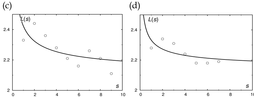
Figure 4: The fitting results. Solid line – fitting function (1), circles – observed data. Panel (a) demonstrates results obtained for the list of types (at fixed c = -1 ), panel (b) corresponds to the whole text, panels (c) and (d) correspond to author's and direct speech, respectively, all at fixed c = -1/2 .
